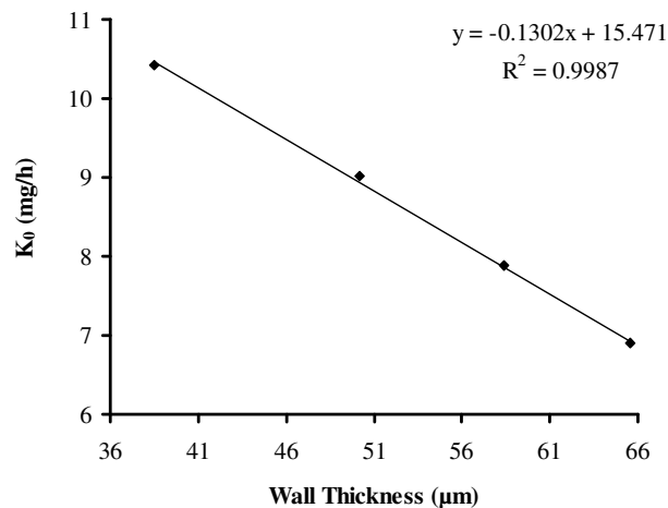
Fig. 2: Relationship between wall thickness and release rate K_0 for HPMC-alginate microcapsules of aceclofenac
