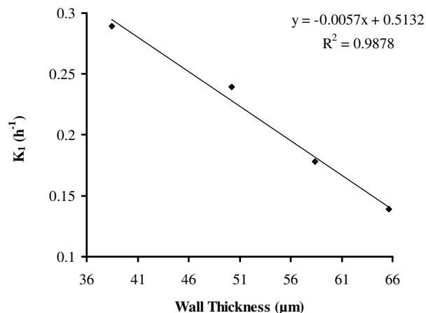
Fig. 3: Relationship between wall thickness and release rate K_1 for HPMC-alginate microcapsules of aceclofenac
