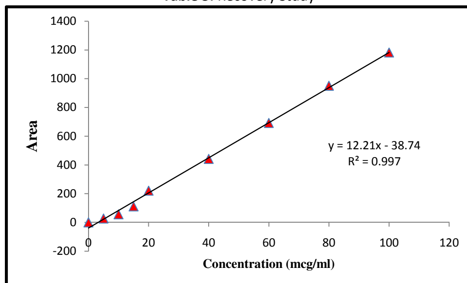
Figure 4: Linearity Plot
