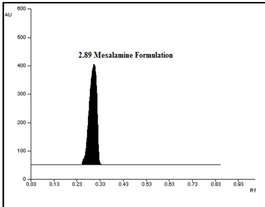
Figure 3: The Chromatogram of 5- ASA Formulation 40 mcg/ml.
