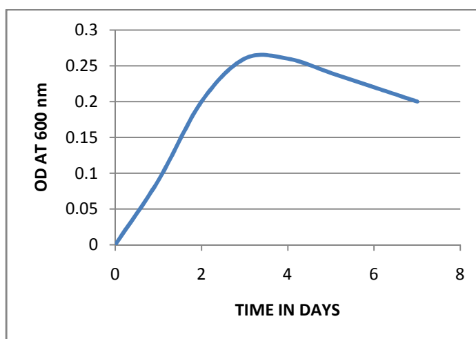
Figure 1: Growth kinetics
