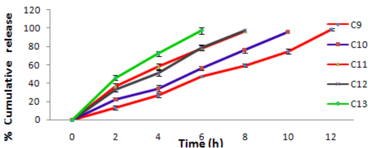
Fig. 3. FMTGR tablets dissolution profile of batches C9 to C13. Mean \pm SD, n = 3
